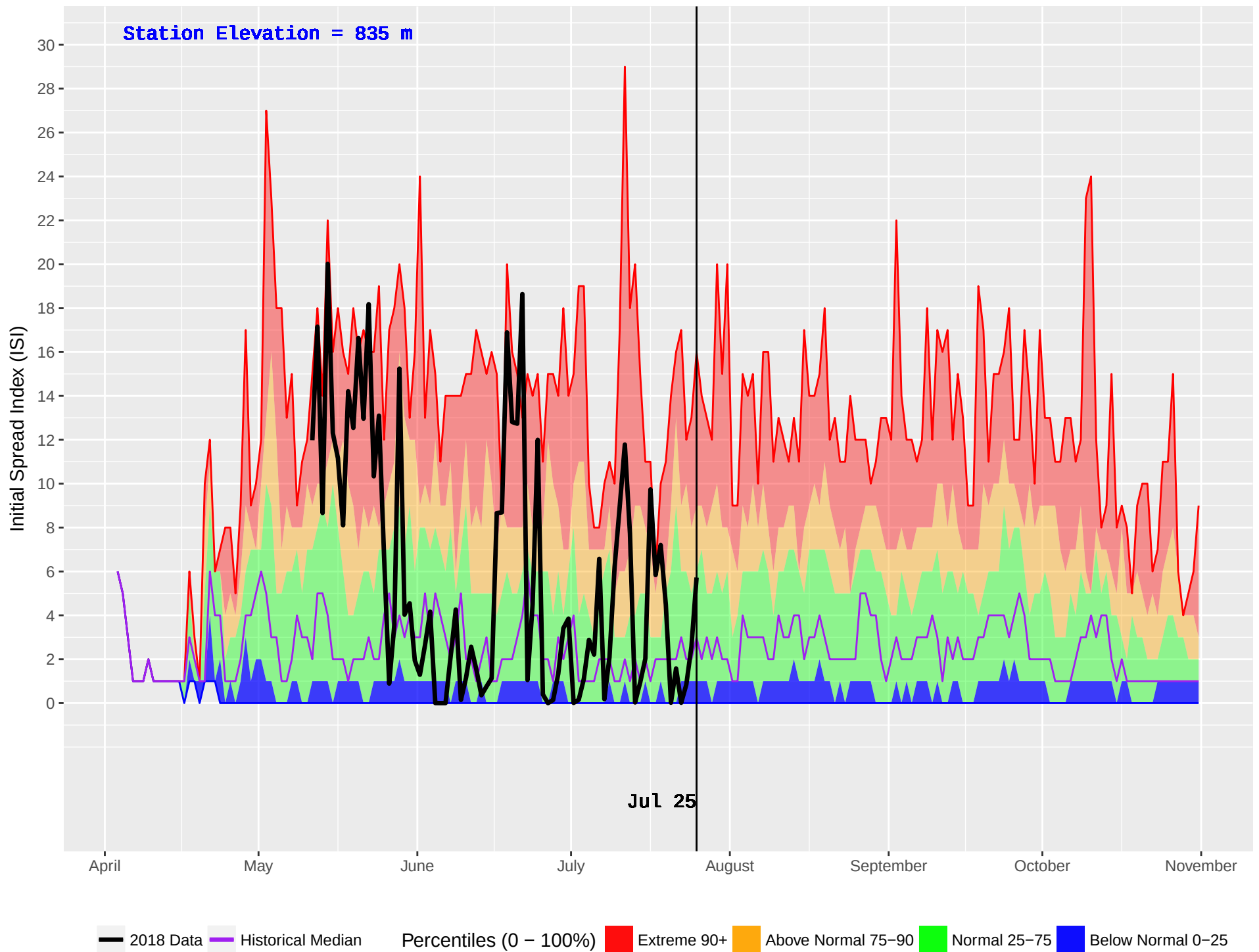
SILVER (120) : Historical (1986–2016) and Current (2018) Noon Initial Spread Index (ISI)
